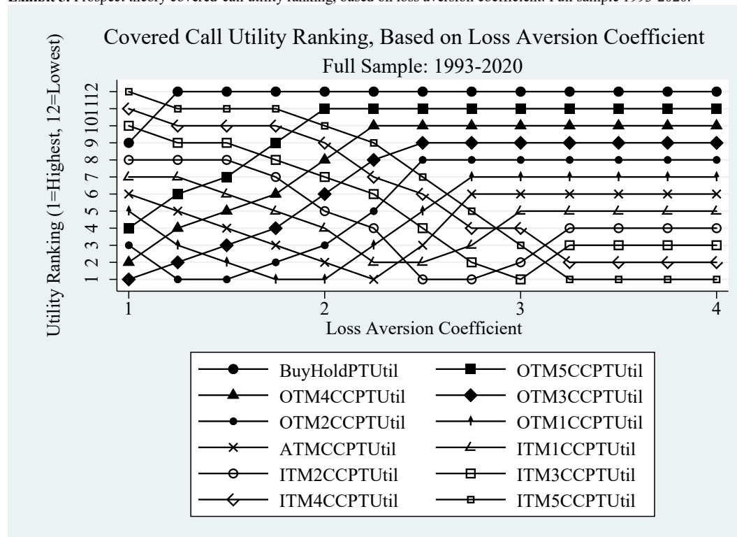
Exhibit 5. Prospect theory covered-call utility ranking, based on loss aversion coefficient: Full sample 1993-2020.
